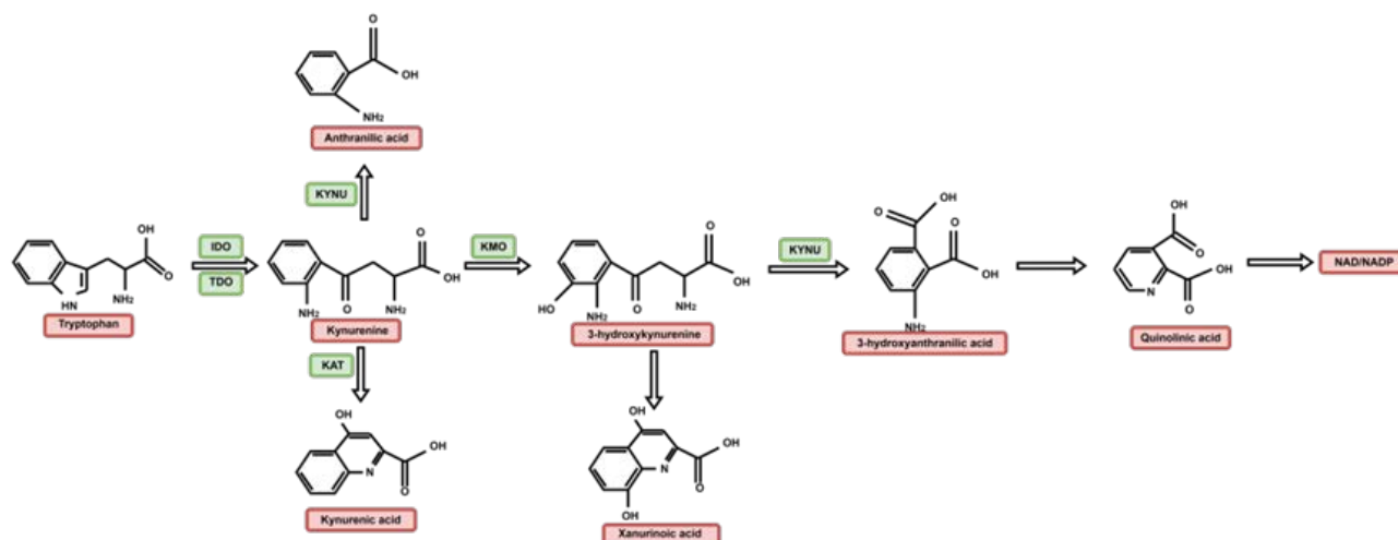
Figure 1. Kynurenine pathway
