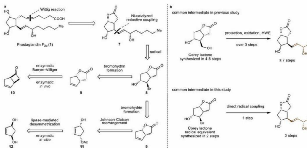
Figure 1 The reverse synthesis process and the [3,3]- \sigma migration (synthesis from 11 to 9)
