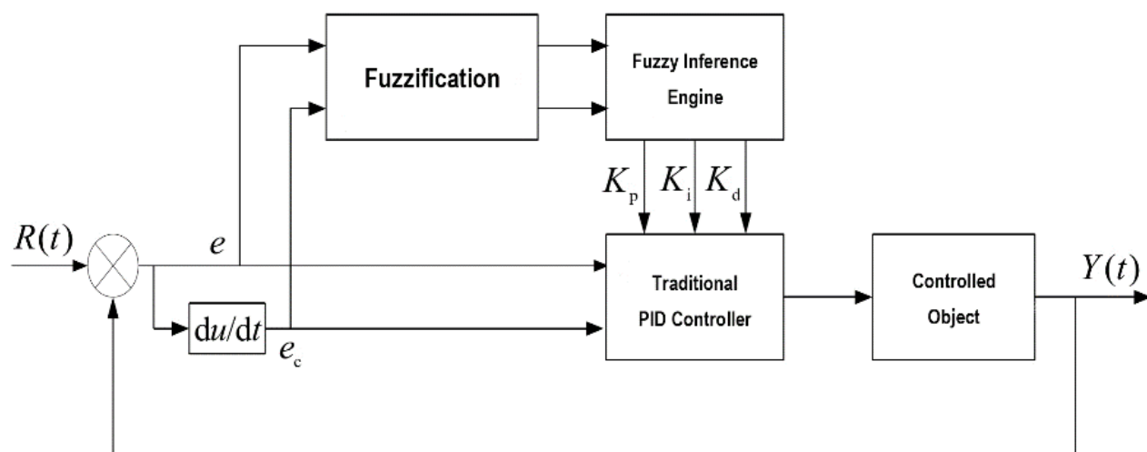
Fig. 3 Fuzzy PID control system structure diagram [7]
